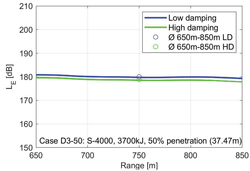
Figure 53: Variation of the predicted L_E for case D3-50 in the range 650m to 850m from the pile for the low and the high soil damping scenario, respectively. Mona upper case pin pile design 5.5m, IQIP S-4000 , hammer energy 3700kJ, pile top flush with sea surface (37.47m) , no sec. noise mitigation.
