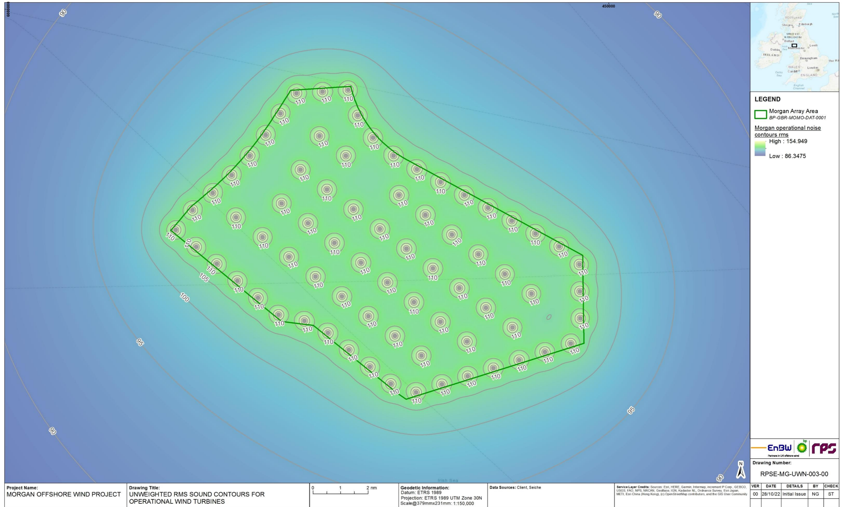
Figure 1.15: Unweighted rms sound contours for operational wind turbines, dB re 1µPa (rms) for an indicative wind turbine generator layout.
