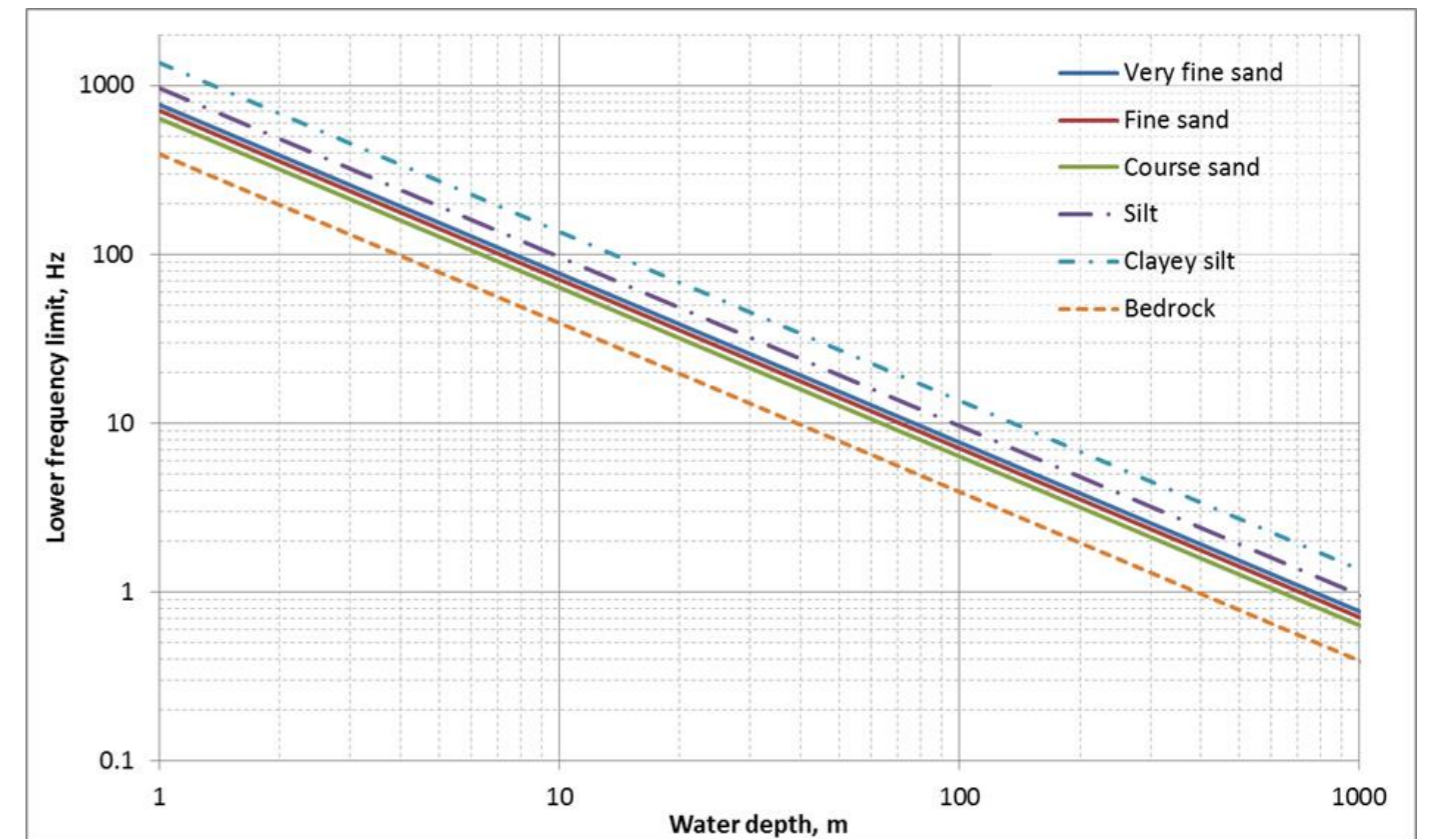
Figure 1.11: Lower cut-off frequency as a function of depth for a range of seabed types
