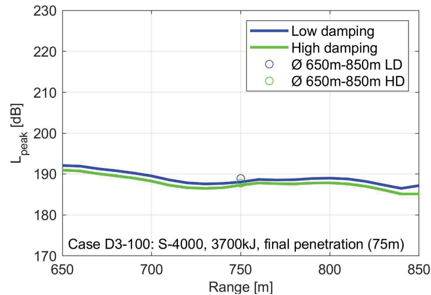
Figure 60: Variation of the predicted L_{peak} for case D3-100 in the range 650m to 850m from the pile for the low and the high soil damping scenario, respectively. Mona upper case pin pile design 5.5m, IQIP S-4000 , hammer energy 3700kJ, final penetration depth (75m) , no secondary noise mitigation.
